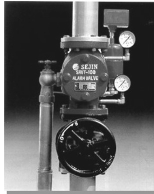
[알람 밸브]
